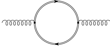
Fig. 3.1. Heavy quark loop graph, which vanishes in the effective theory. Heavy quark propagators are denoted by a double line.
